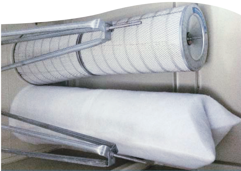
Single piece design of GDX/GDS cartridge wrap allows for easy installation and change out during operation. For use with any GDX/GDS conical, cylindrical cartridge/canister filter
